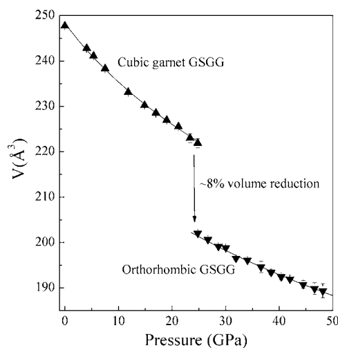
Figure 5. Experimental P - V data of the garnet and high-pressure orthorhombic perovskite phases GSGG. The solid line is the fit with the Birch-Murnaghan EOS for the P - V data.
